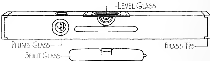
FIG. 32 . PLUMB AND LEVEL.
